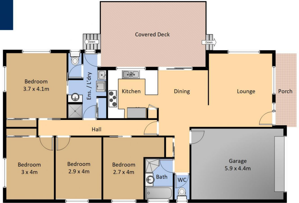
Main Level
