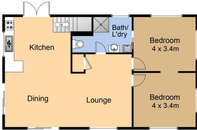
Ground Level
